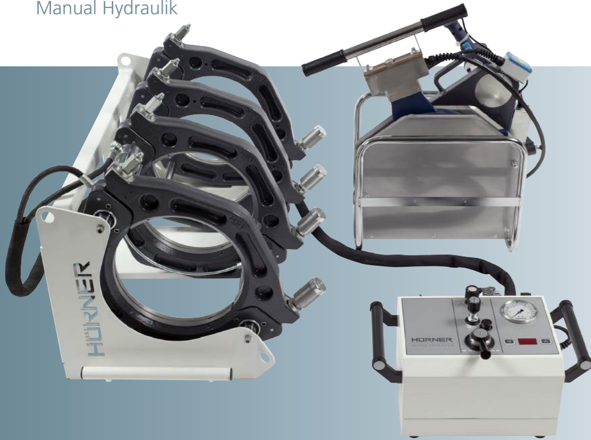
Stand-alone in Butt-Welding
